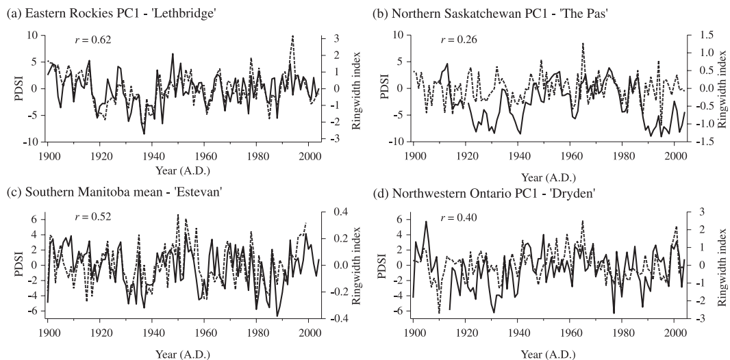
FIG. 5. Time series for instrumental PDSI (solid lines) and regional ring width (dashed lines) with the interseries correlations (“ r ”): (a) eastern Rockies PC1, (b) northern Saskatchewan PC1, (c) southern Manitoba mean, and (d) northwestern Ontario PC1.
