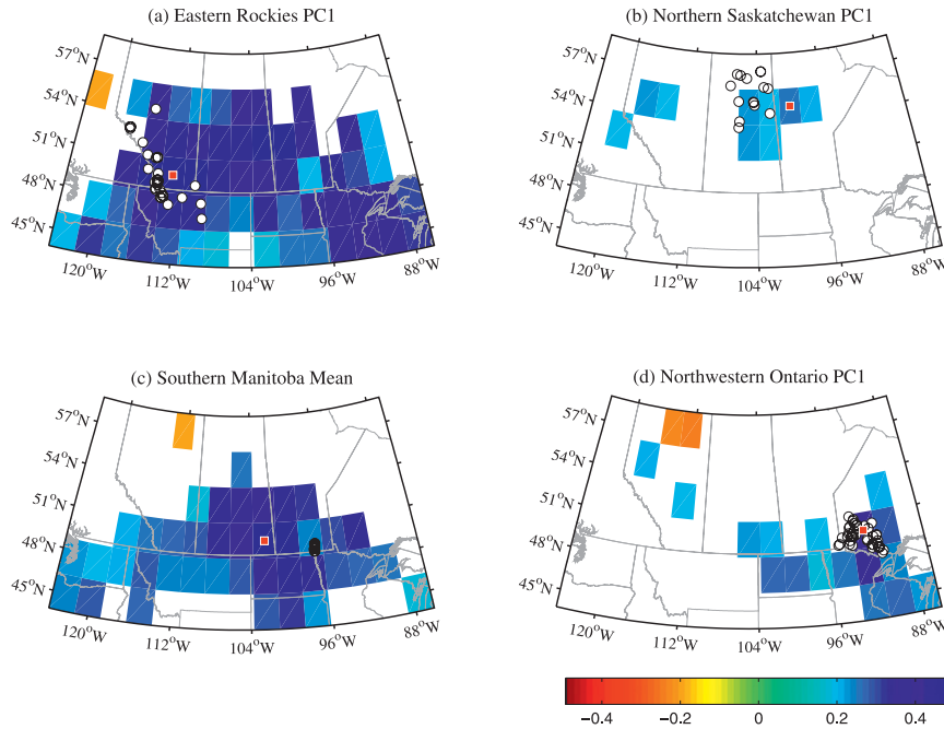
FIG. 4. Correlations between regional ring-width indices and gridded July PDSI. Only correlations that are significant at the 0.05 level are shown. Red squares mark grid points with the highest absolute correlation between regional ring width and PDSI. The period of analysis is 1900–2002.
